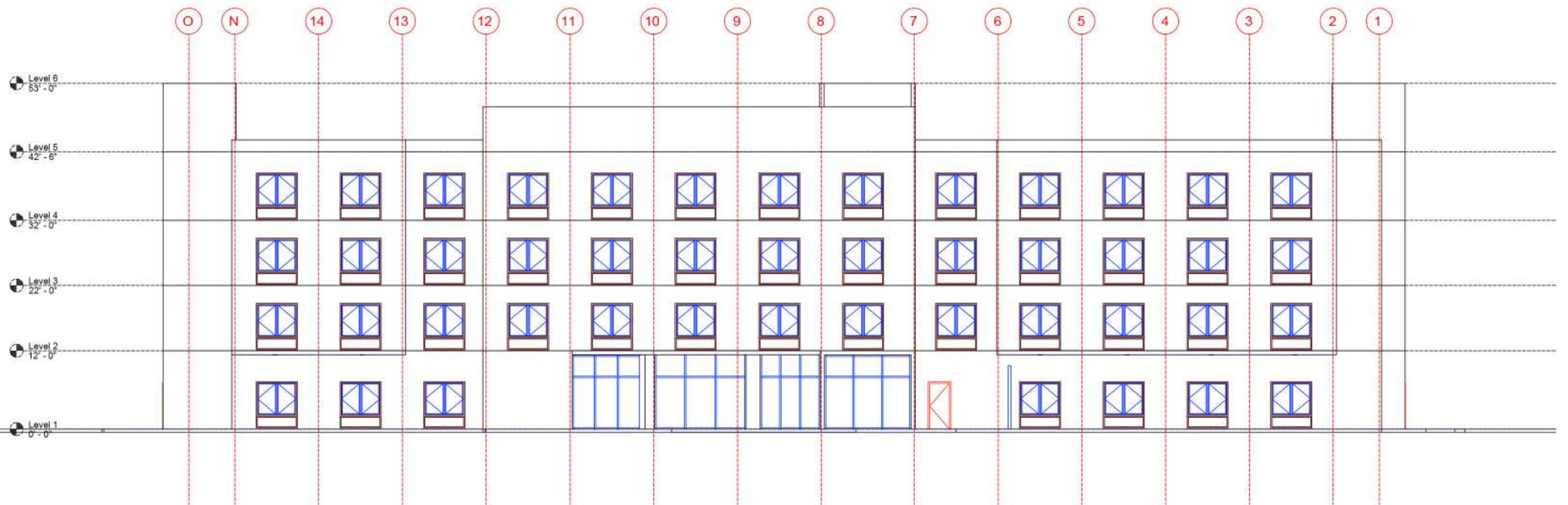
HOTEL BACK ELEVATION
