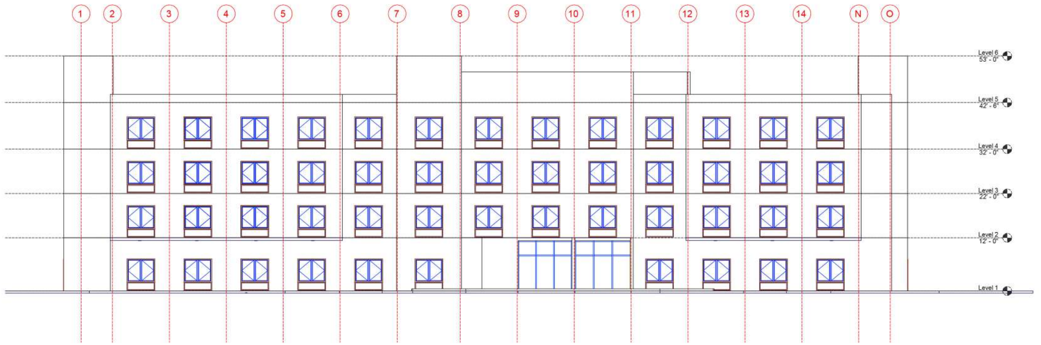
HOTEL FRONT ELEVATION
